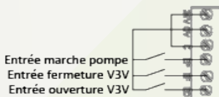
3.1. Commande contact sec
